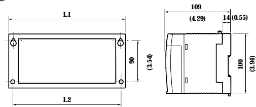
Figure 9.2 External dimensions
